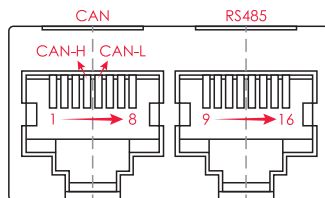
CAN and RS485 interfaces
